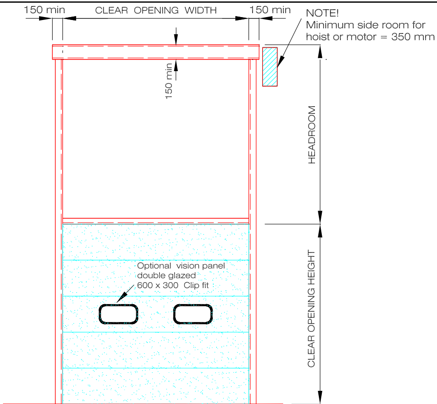
ELEVATION OF PREPARED OPENING VIEWED FROM INSIDE
